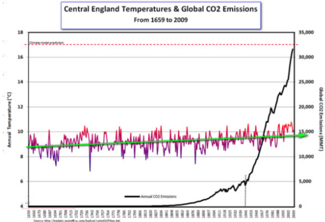
1659–2009 Temperature and Carbon Dioxide Emissions in Central England. (Courtesy of Patrick Moore)
